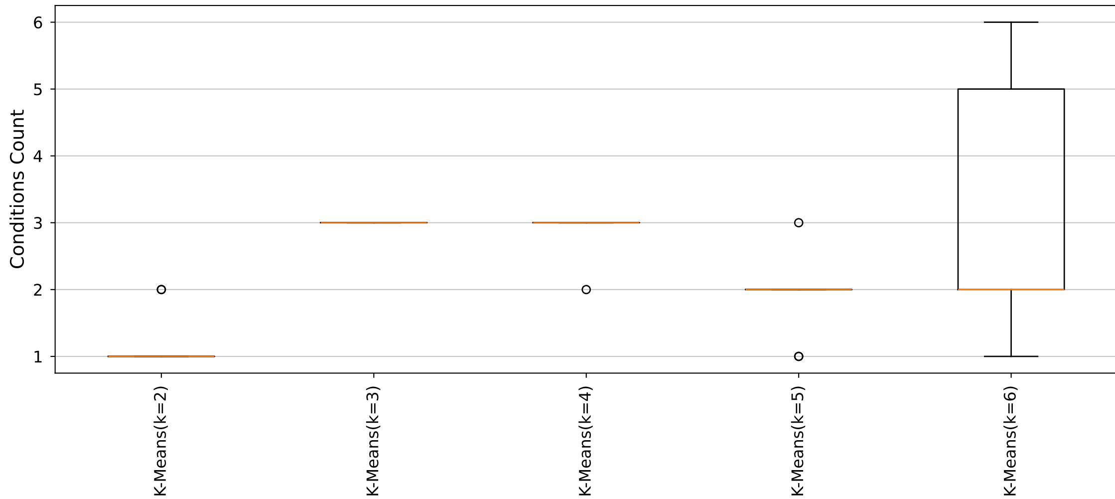
YARA Rules Conditions Count Distribution (Cluster33_Size6 dataset)
